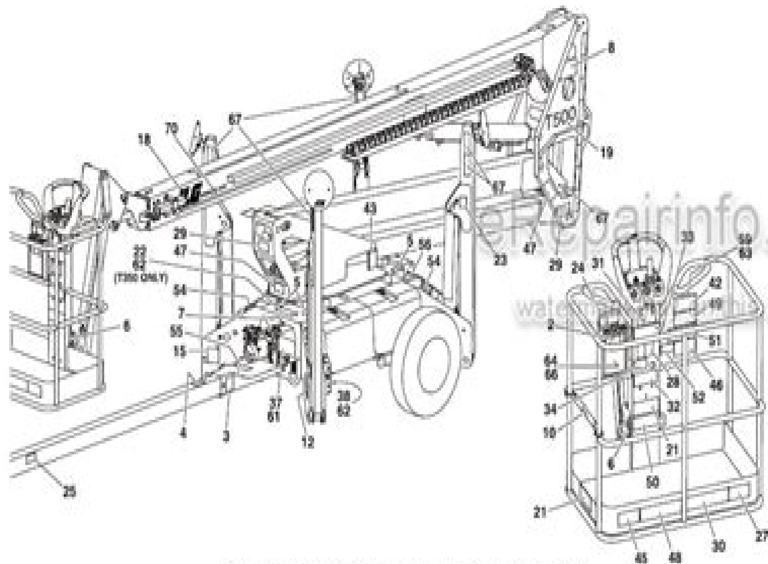
Figure 5-14. Decal Location - Country Specs (Sheet 1 of 2)
