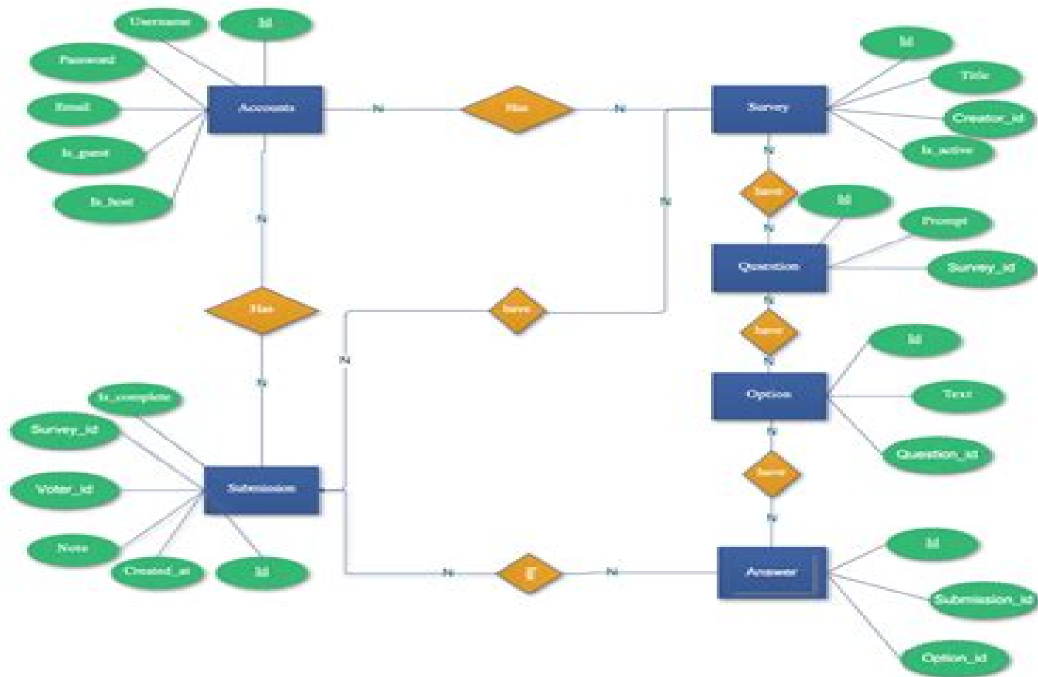
ER diagram for web_based gathering voting system
