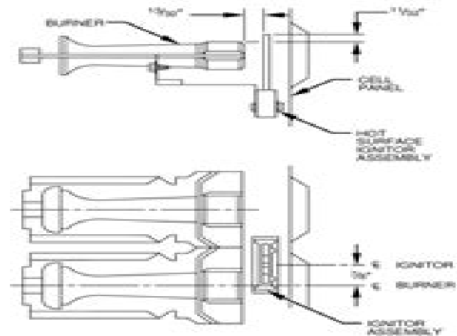
Fig. 9—Position of Ignitor to Burner
