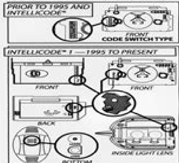
FIG. 1. POWERHEADS (for various models) Circle shows location of Learn Code Button and LED.
