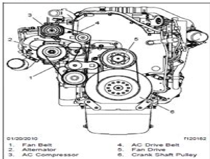
Fig. 1, Cummins ISX Drive Belt Routing
