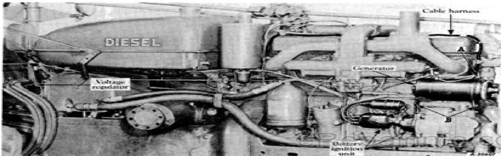
Illustr. 58 Generator, battery ignition unit, cables, etc.
