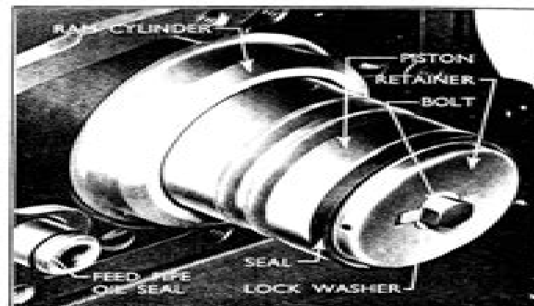
Fig. 196 Fitting the Ram Cylinder Piston
