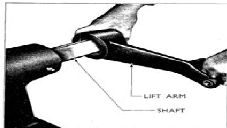
Fig. 195 Fitting a Lift Arm
