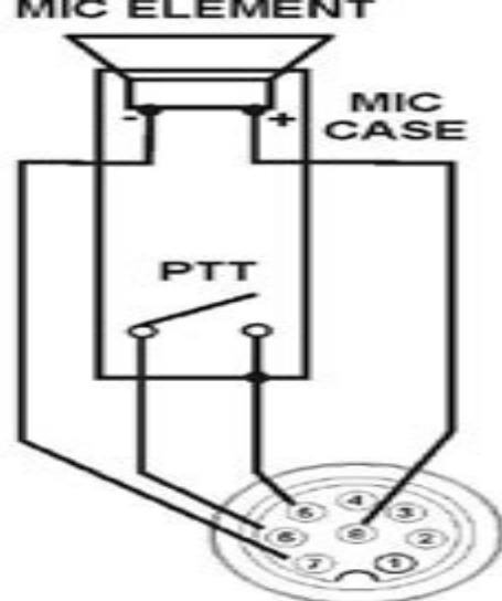
TRANSCEIVER MICROPHONE JACK FRONT VIEW
