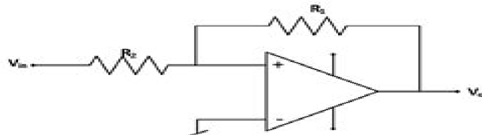
FIG. 7.2 Schmitt Trigger (NONINVERTING MODE)
