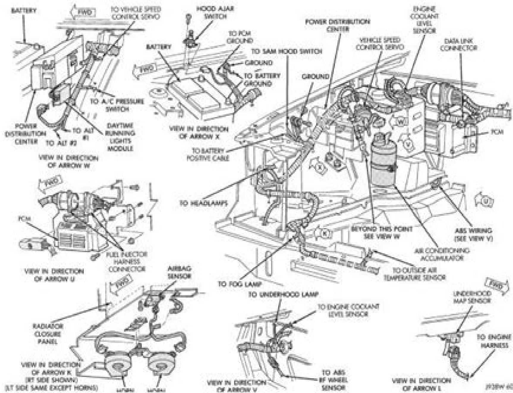
Fig. 13 Engine Compartment Wiring (Right Side)
