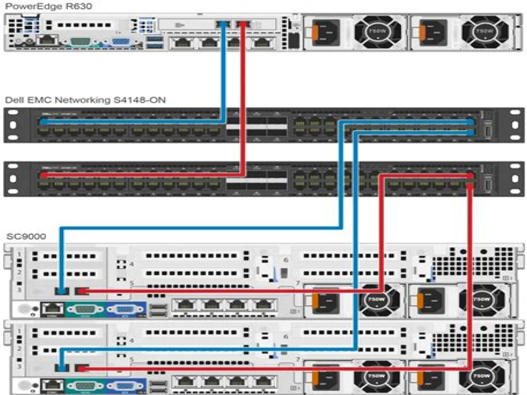
Figure 1 Cabling diagram
