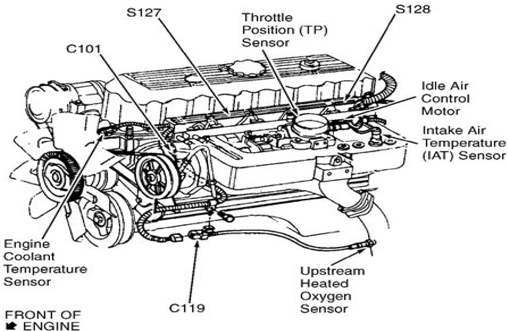
4.0L ENGINE
