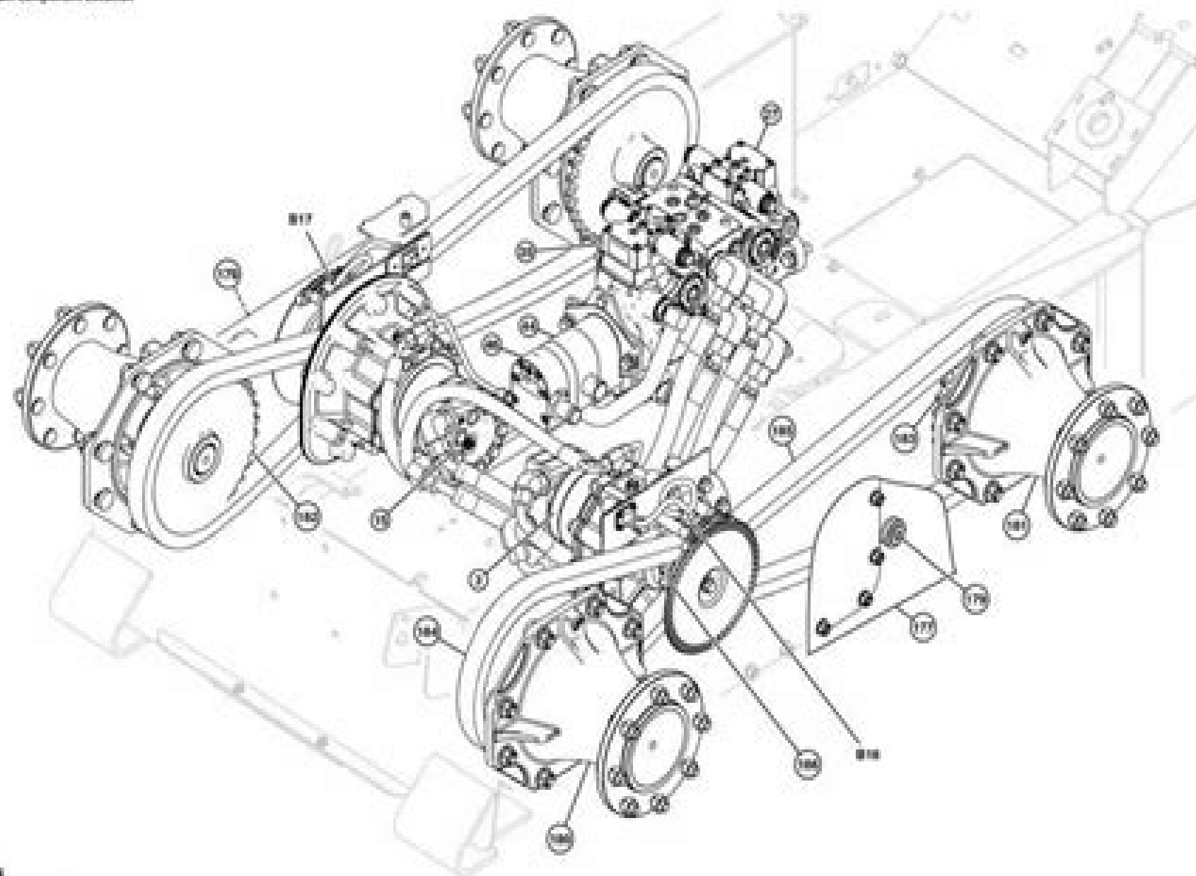
TX1000004 Power Train Component Location (single speed machine shown)
