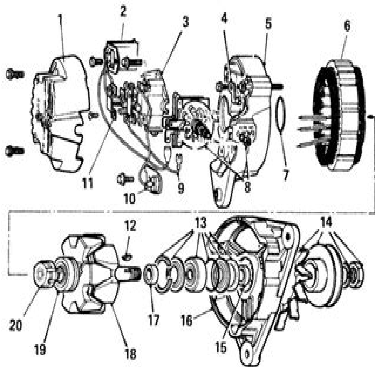
Exploded view of Lucas 16ACR alternator. (Late type with single wiring plug termination shown)
