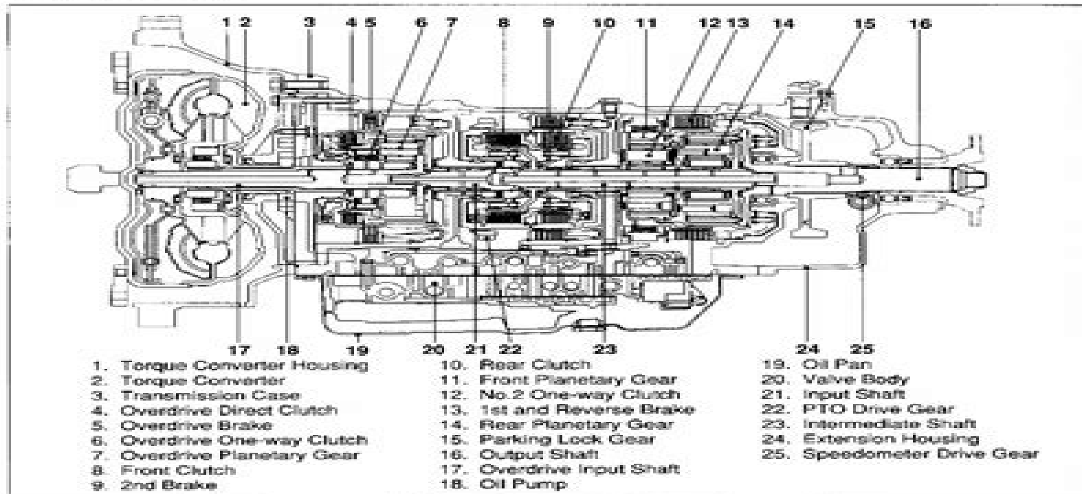
Figure 1. Construction of Automatic Transmission
