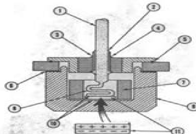
Figure 6 Diode Construction
