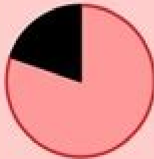
Sector
