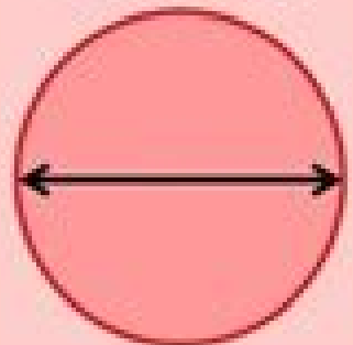
Diameter
