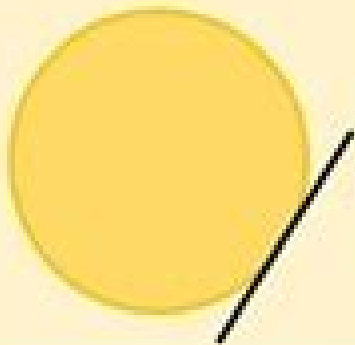
Tangent
