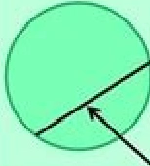
Chord
