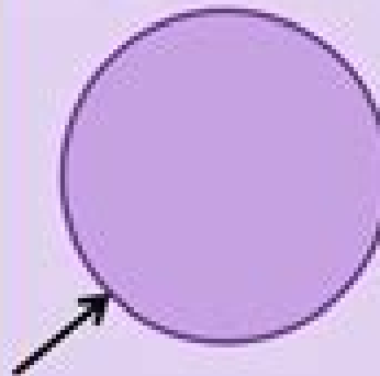
Circumference
