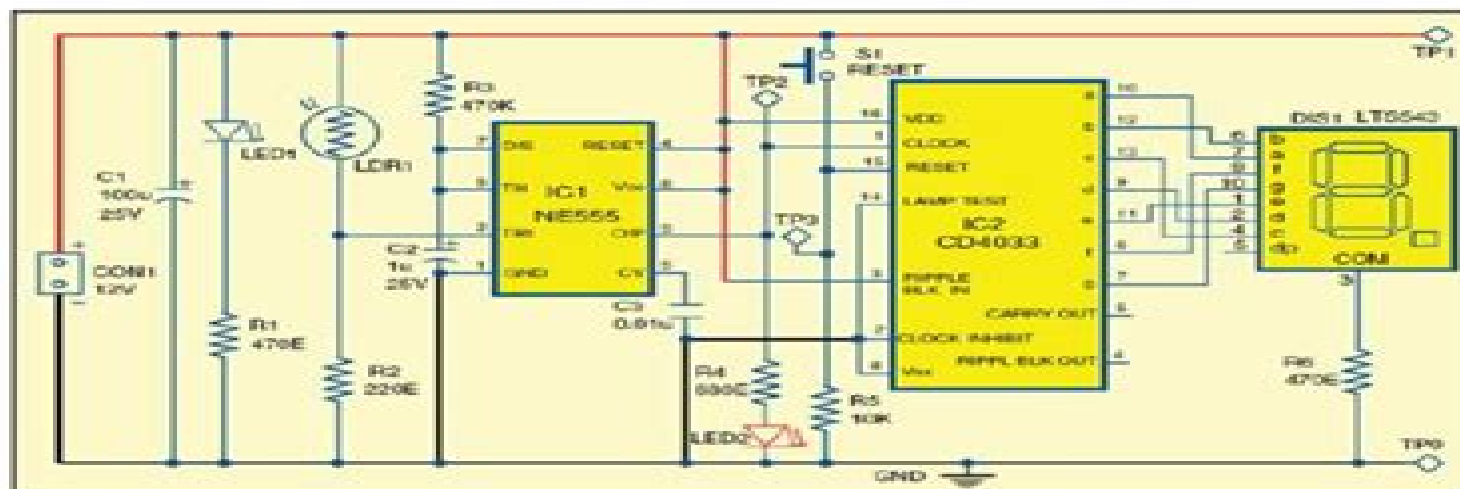
Fig. 2: Circuit diagram of the electronic letterbox with letter-counting facility
