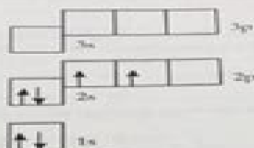
Carbon 1s^2 2s^2 2p^2
