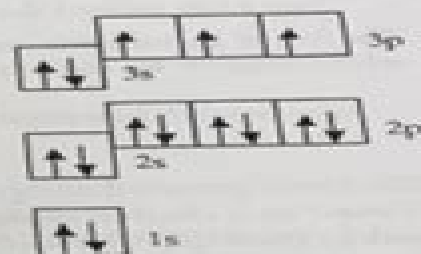
Phosphorus 1s^2 2s^2 2p^6 3s^2 3p^3
