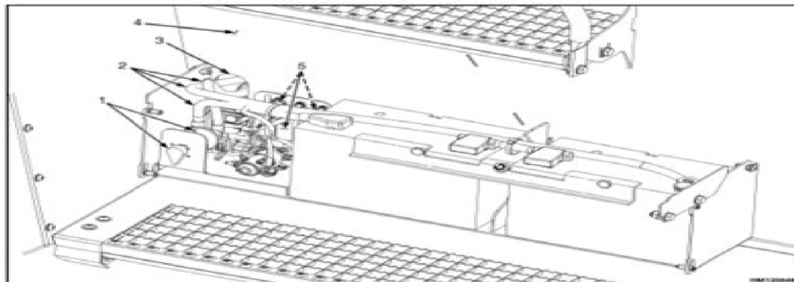
Figure 13. Fuel Tank Cable Hole
