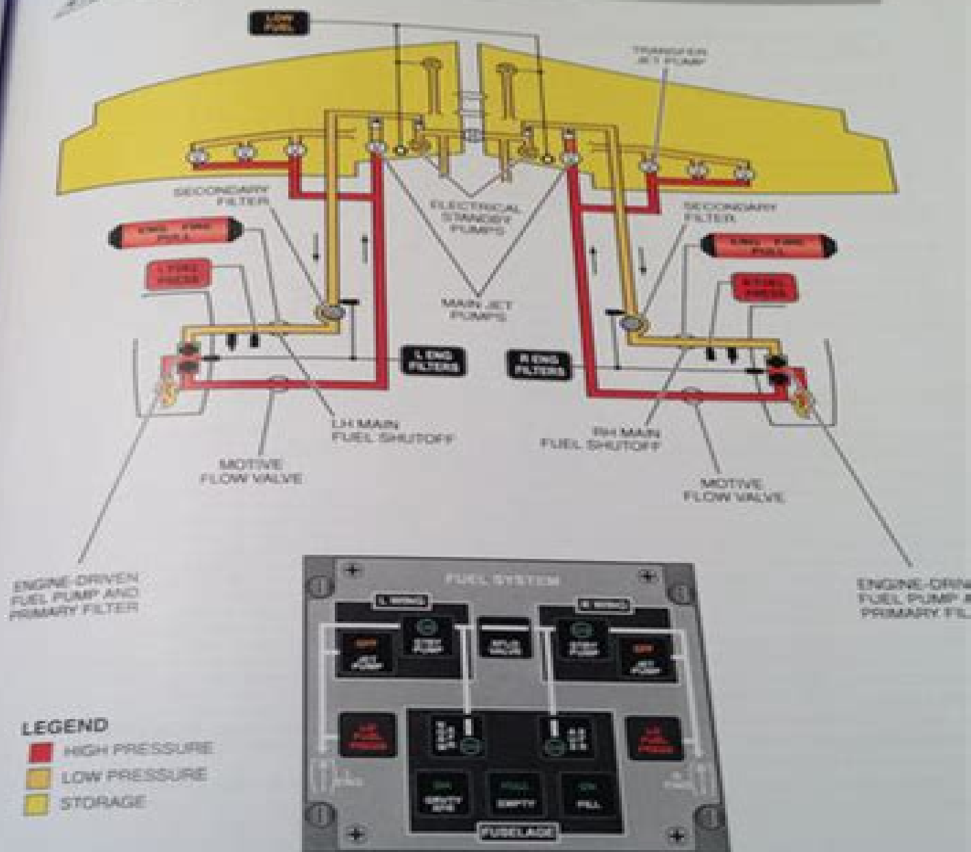
Figure 5-10. Engine Fuel Supply Schematic
