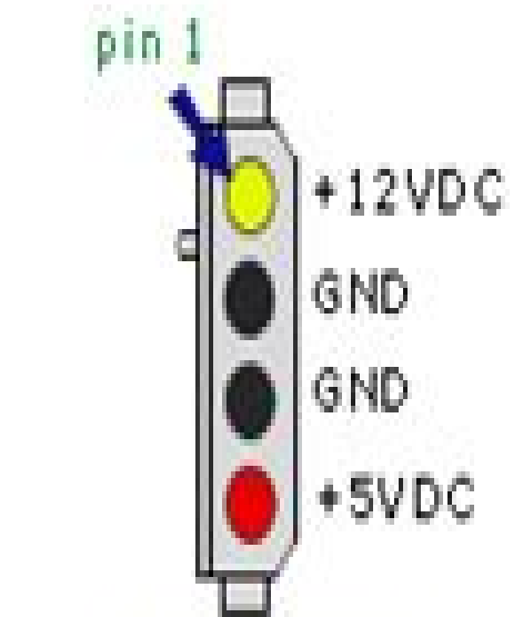
4 pin Molex peripheral Connector
