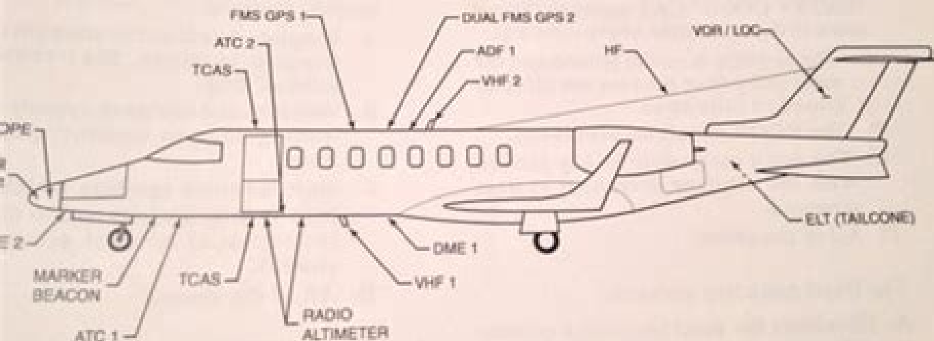
Figure 1-21. Airplane Antennas
