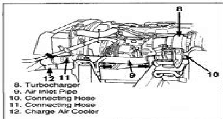
Figure 4. Air Inlet Pipe Attachment
