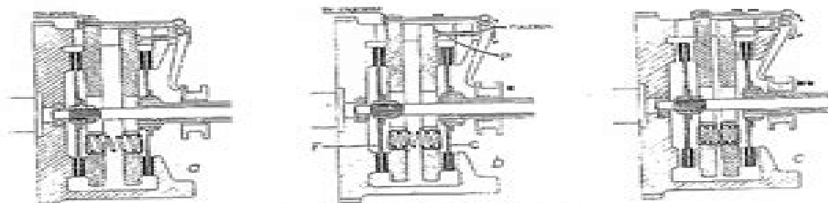
Fig. 82. - Clutch functional diagram.
