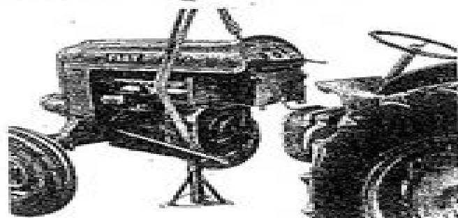
Fig. 83. - Removal of engine, with front axle.
