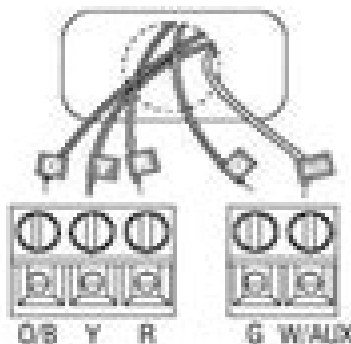
Heat Pump Systems with Auxiliary/Backup Heat (Typical Wiring)
