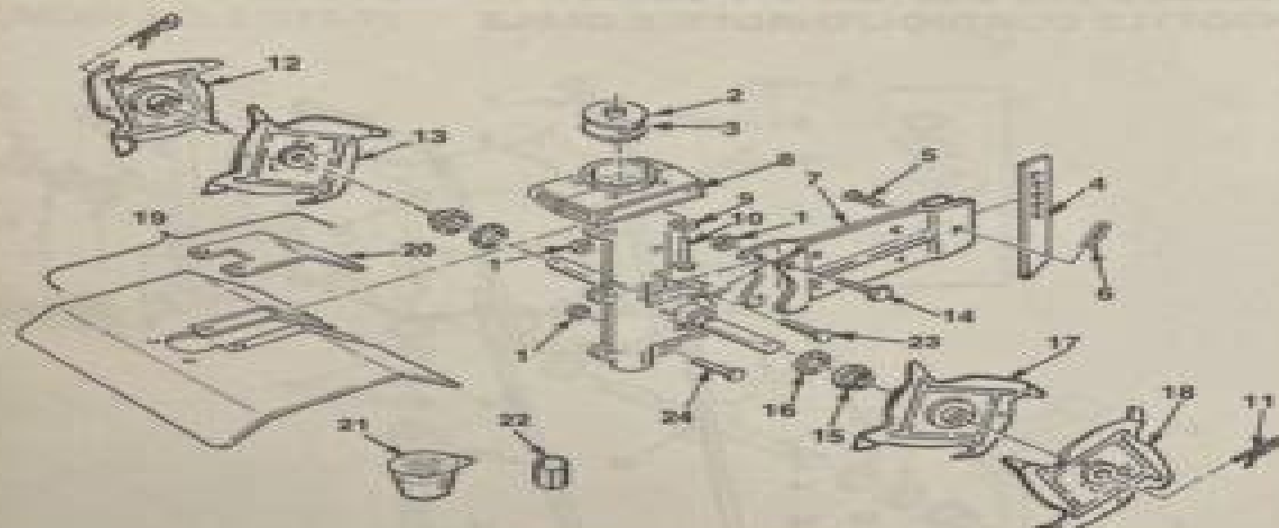
FIGURE 3 ENGINE/TRANSMISSION/TINES/SHIELD
