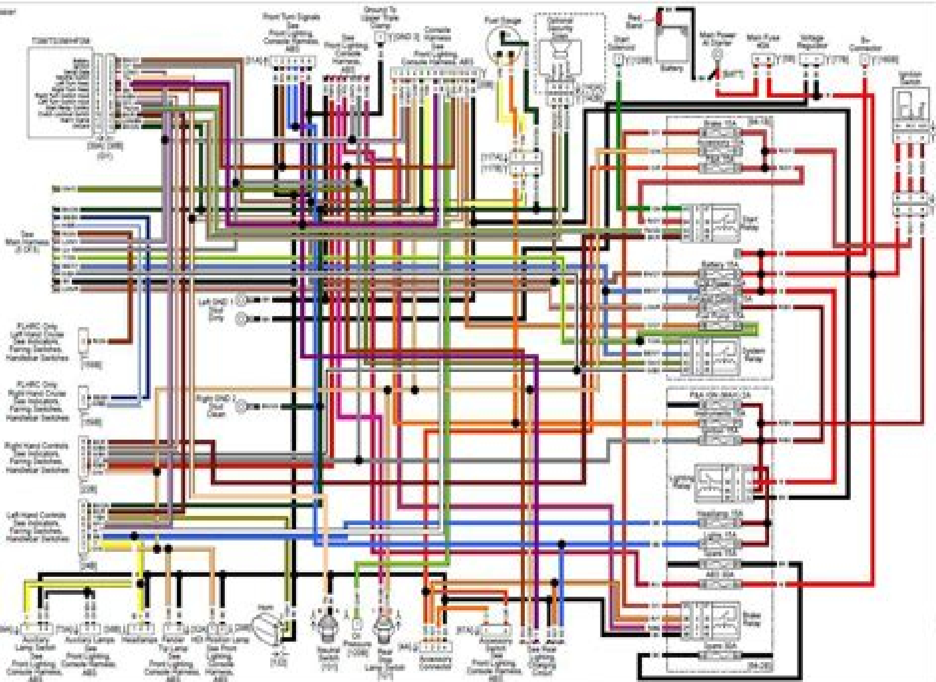
Figure 6-17. MAIN HARNESS (A OR B) 2004 Touring (FLHRC) with ABS
