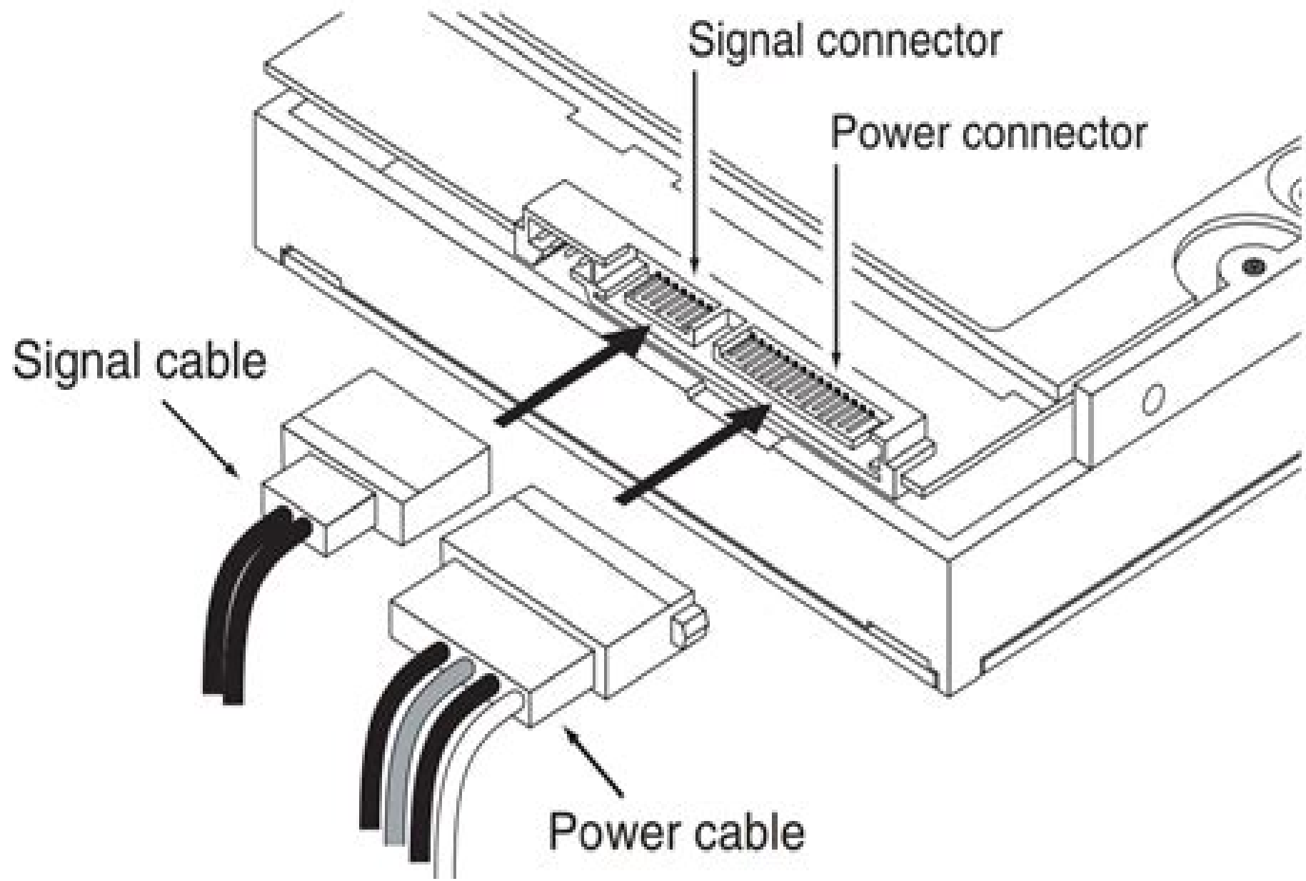
Figure 1 Attaching SATA cabling
