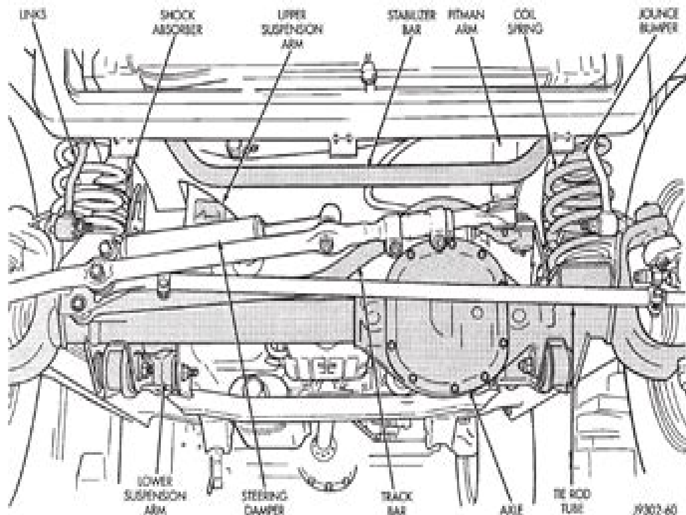
Fig. 1 Front Suspension
