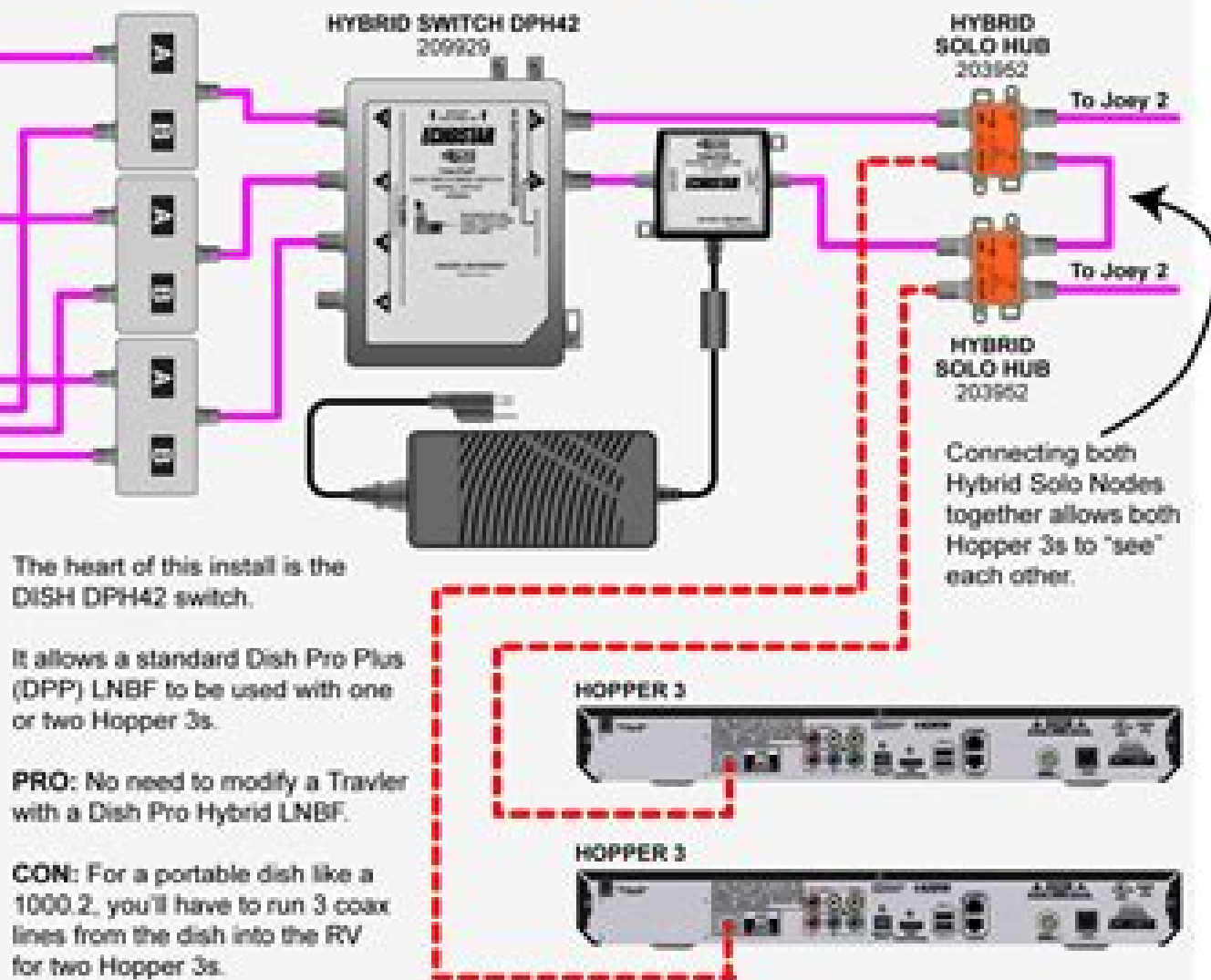
DISH 1000.2 with DPP LNB
