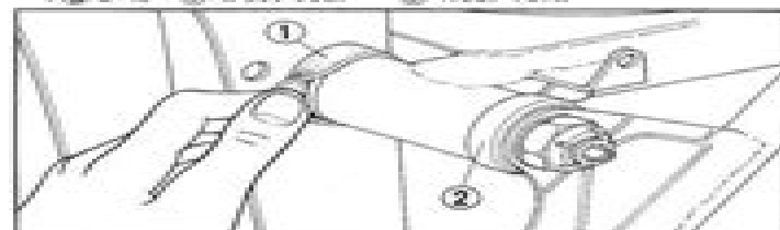
Fig. 2-50 ① Dust seal ② Rear fork
