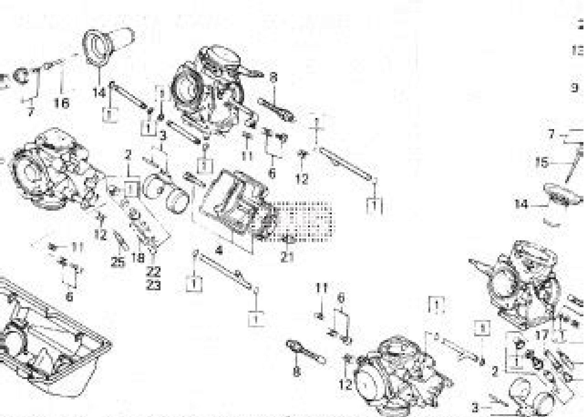
E-17-1 CARBURETOR (COMPONENT PARTS)
