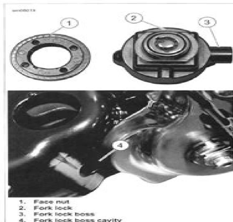
Figure 2-166. Fork Lock
