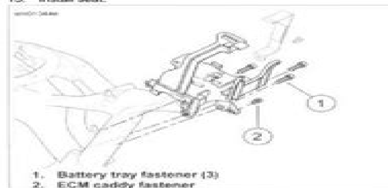
Figure 6-18. Battery Tray
