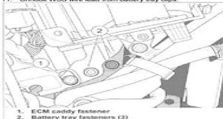
Figure 6-17. Battery Tray Fasteners
