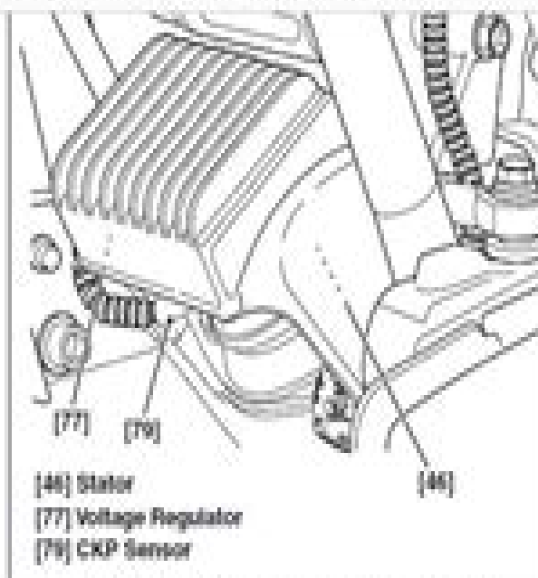
Figure 9-5. Voltage Regulator (Left Side View)
