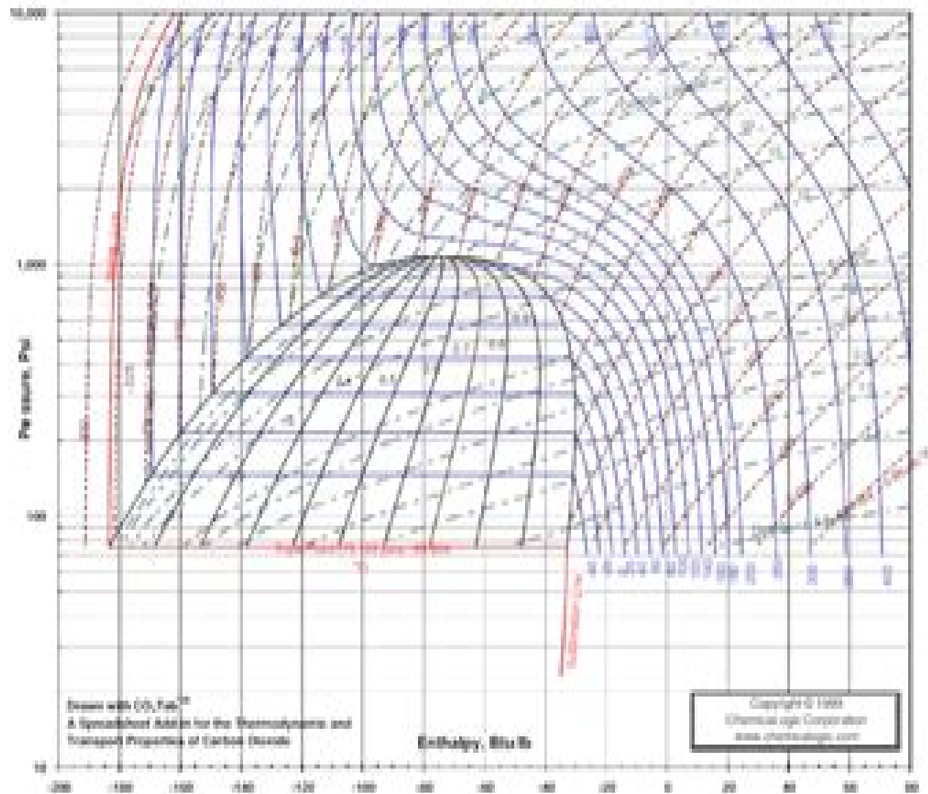
Carbon Dioxide: Pressure - Enthalpy Diagram
