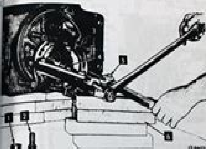
Diagram 10 Removing the Bend-Piston
