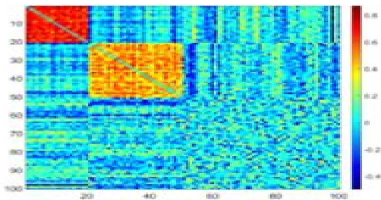
(a) A weighted network with explicit structures
