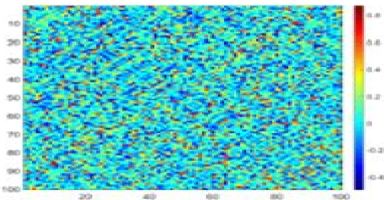
(b) A random weighted network/ graph
