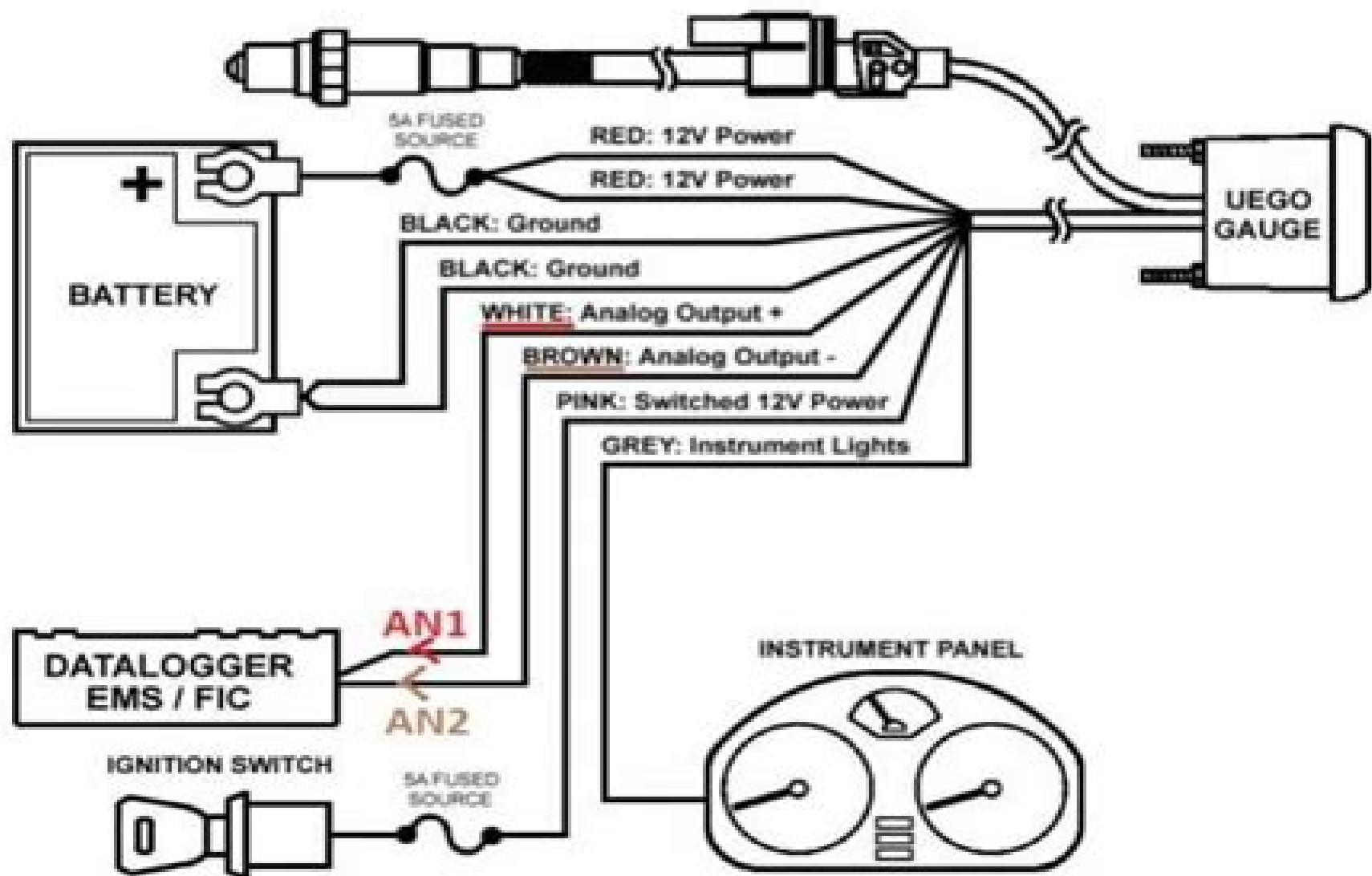
Figure 1. Wiring Schematic
