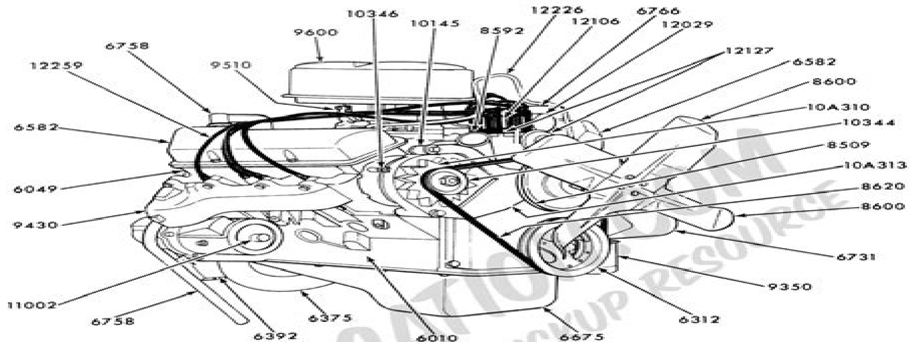
RIGHT-FRONT VIEW
