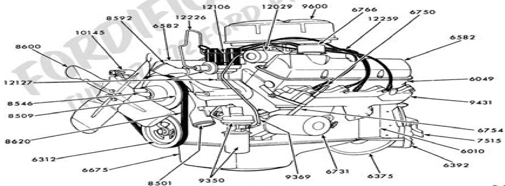
LEFT-FRONT VIEW
