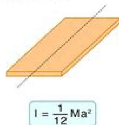
Rectangular plate with axis passing parallelly through the center
