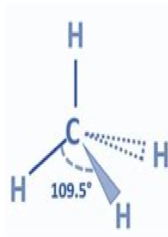
Molecular geometry of CH 4
