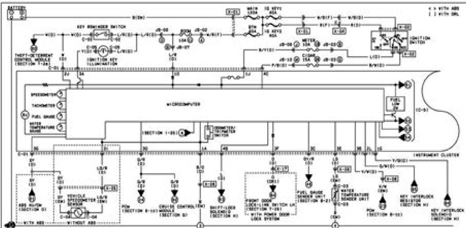
C-21 INSTRUMENT CLUSTER (2)
