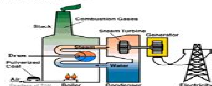
Fig. 1. General diagram of boiler-turbine unit.
