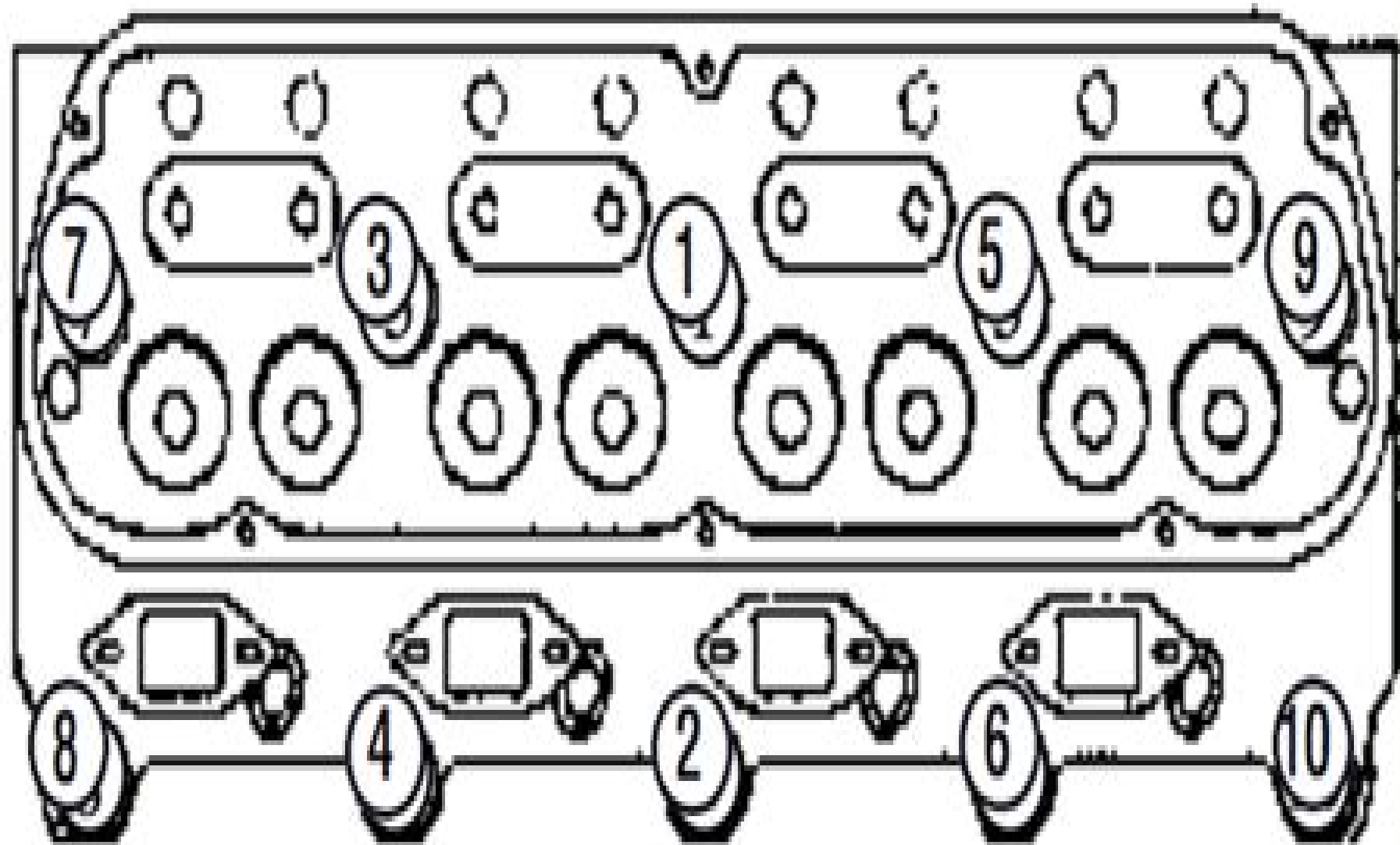
Figure 1—Tightening Sequence
