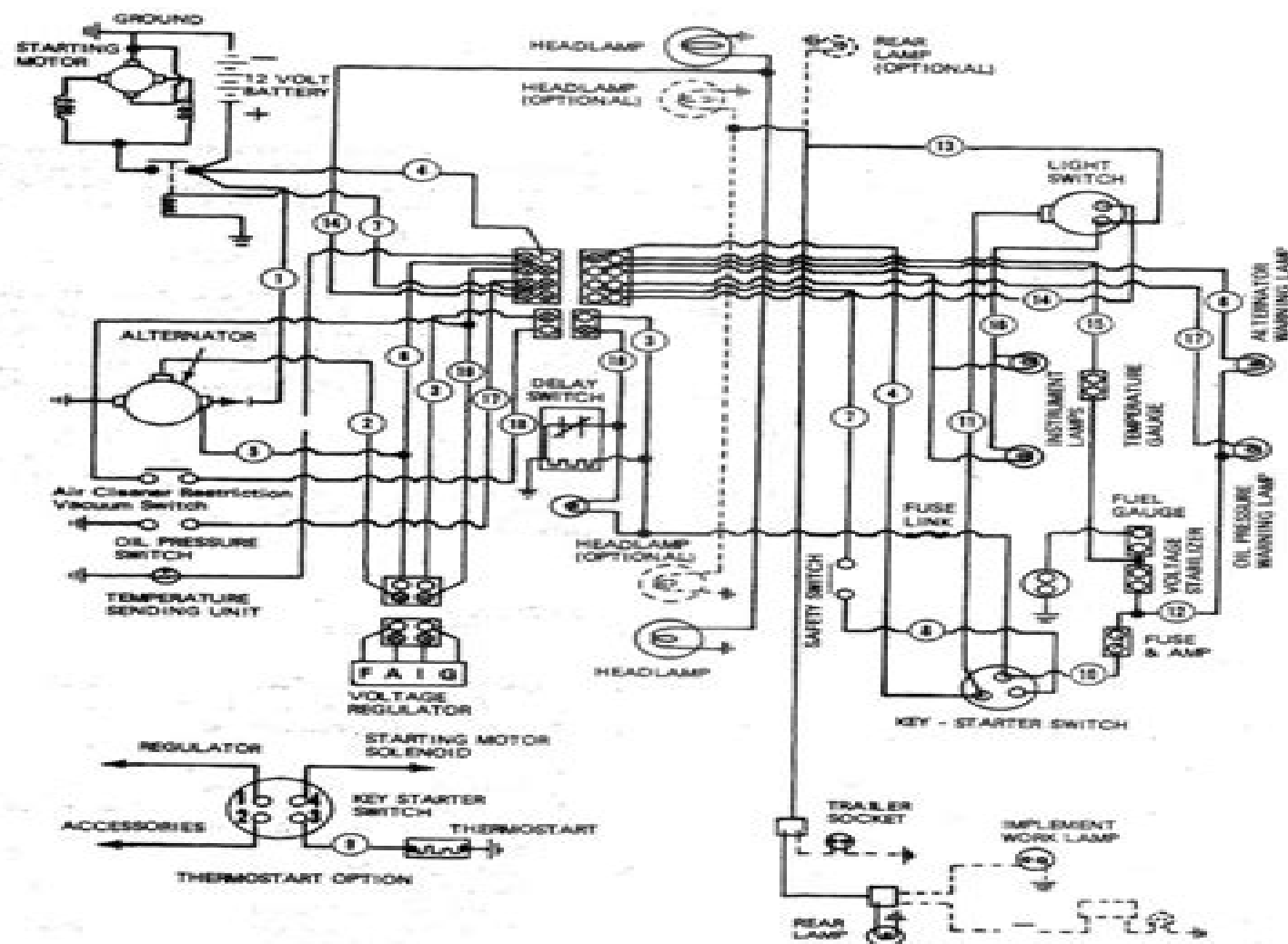
Figure 1 Electrical System Schematic
