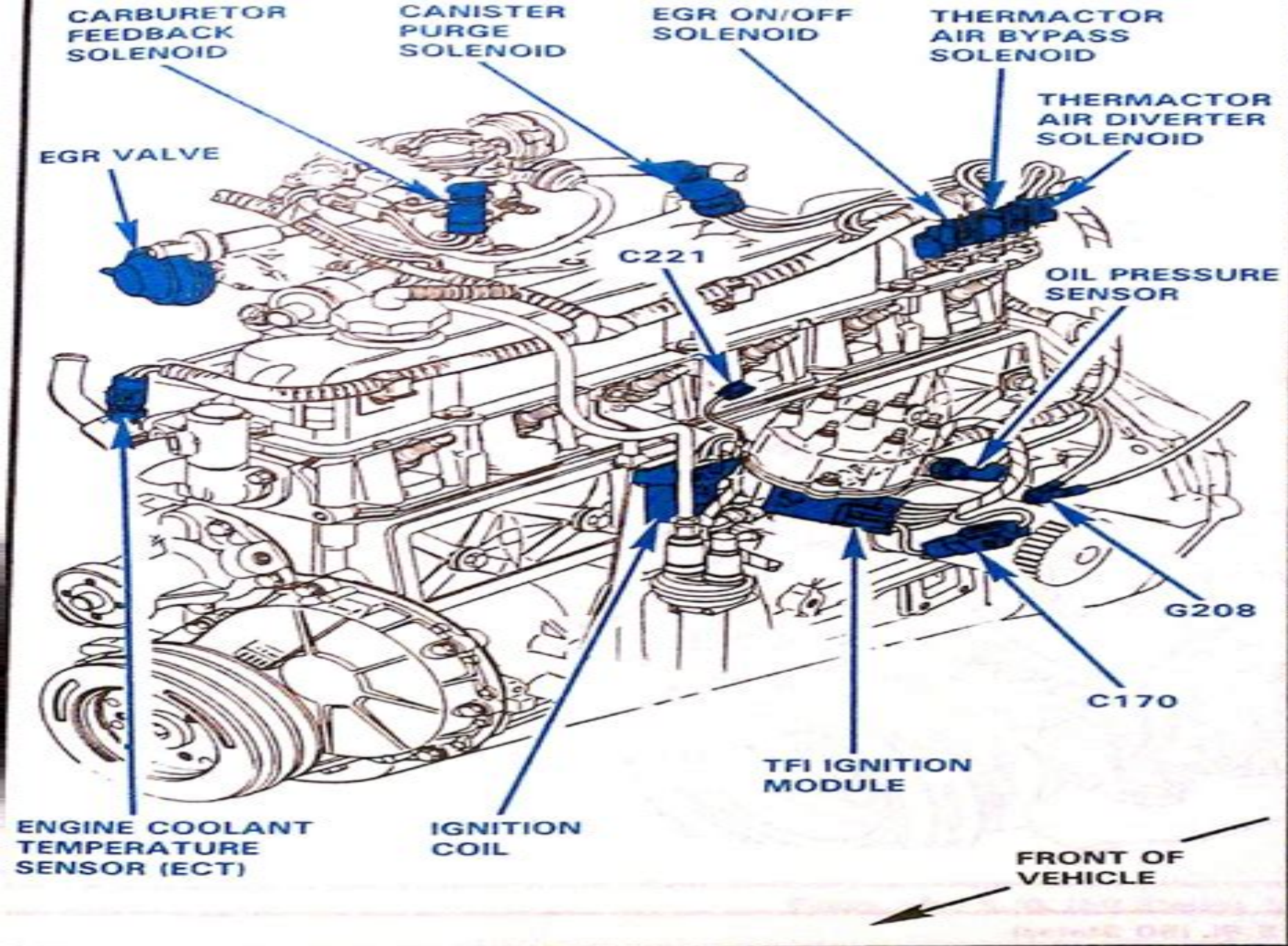
Figure 16 — LH View 4.9L Engine (50 States) Under 8500 lbs. GVW (EEC IV)
