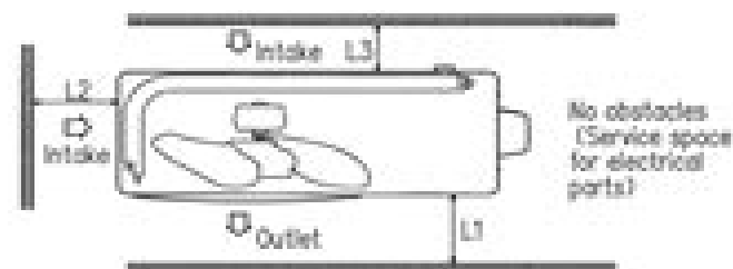
Minimum installation space
